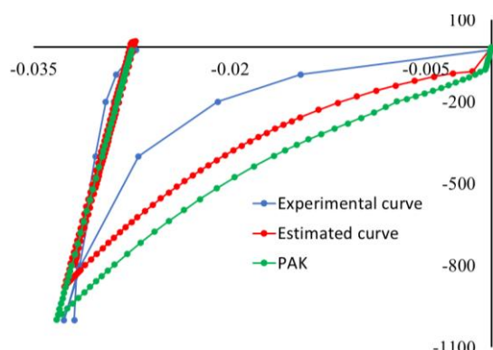
Fig. 7. Results of numerical simulation of oedometer test 3
